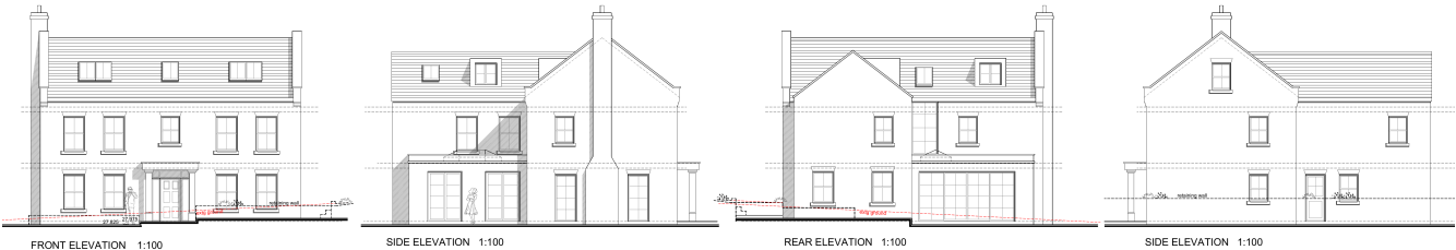
APPROVED ELEVATIONS — FRONT, SIDE, REAR AND SIDE (DRAWING 021 REV C)
